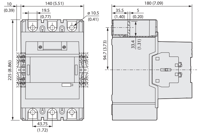
Figure 84 - 100-E265...100-E370 Contactors
