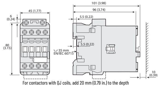
Figure 44 - 100-E26...100-E38 4-Pole Contactors with Standard Coils
