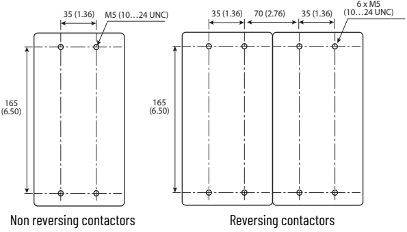
Figure 84 - 100-E265...100-E370 Contactors
