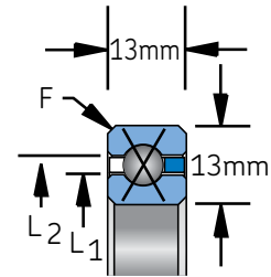
Snap-over separator 1/4" (inch) balls 4 Point Contact Type X
