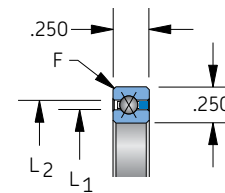
Snap-over separator 1/8" balls
