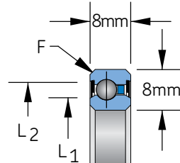
Snap-over separator 5/32" (inch) balls Conrad Assembly Type C
