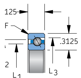
Circular pocket separator 5/32" balls
