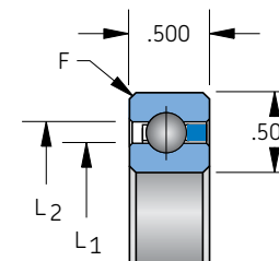
Snap-over separator 1/4" balls
