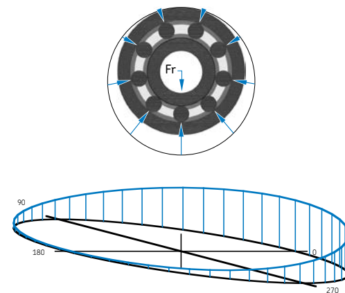
KA040CPOK with 100 lbs. radial load Light preload in the bearing; all balls carry the load.
