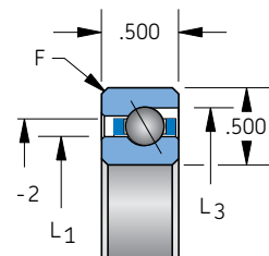
Circular pocket separator 1/4" balls
