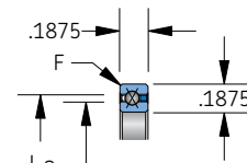
Snap-over separator 3/32" balls
