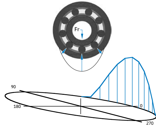
KA040CP0 with 100 lbs. radial load Clearance in the bearing; few balls carry the load.
