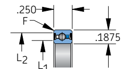
Snap-over separator 3/32" balls
