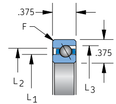
Circular pocket separator 3/16" balls
