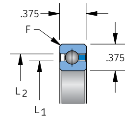
Snap-over separator 3/16" balls
