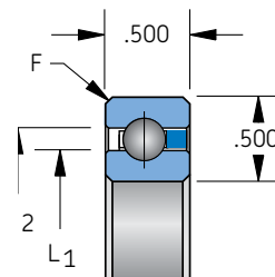
Snap-over separator 1/4" balls
