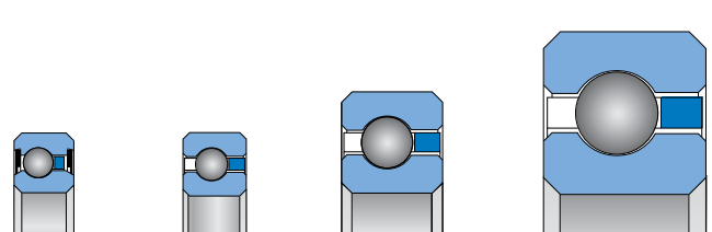
Sealed 8mm x 8mm Open 8mm x 8mm Open 13mm x 13mm Open 20mm x 20mm
