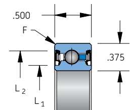
Snap-over separator 3/16" balls
