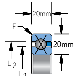
Snap-over separator 3/8" (inch) balls 4 Point Contact Type X
