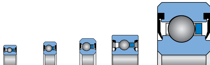
Series JHA \frac{3}{16} " x \frac{1}{4} " Series JA \frac{1}{4} " x \frac{1}{4} " Series JB \frac{5}{16} " x \frac{5}{16} " Series JU \frac{1}{2} " x \frac{3}{8} " Series JG 1" x 1"
