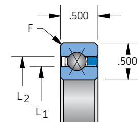
Snap-over separator 1/4" balls
