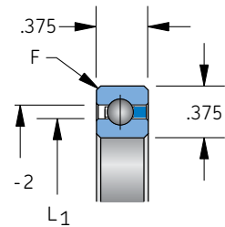
Snap-over separator 3/16" balls
