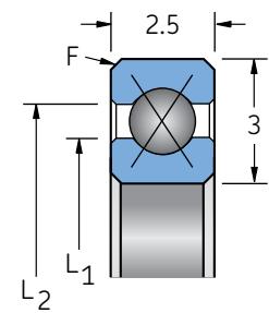
Full complement or spacer ball 1/16" (inch)
