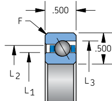
Circular pocket separator 1/4" balls
