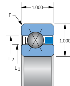
Snap-over separator 1/2" balls
