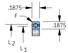
Snap-over separator 3/32" balls
