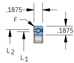
Snap-over separator 3/32" balls
