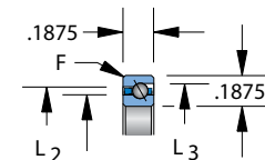
Circular pocket separator 3/32" balls
