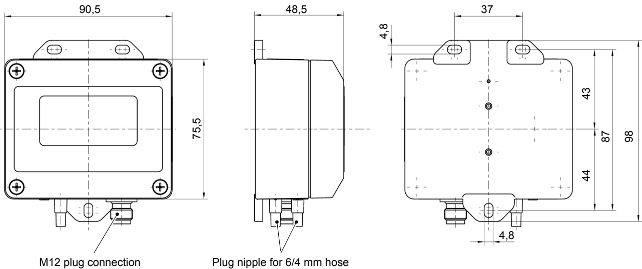
Illustration 4: Dimensional drawing
